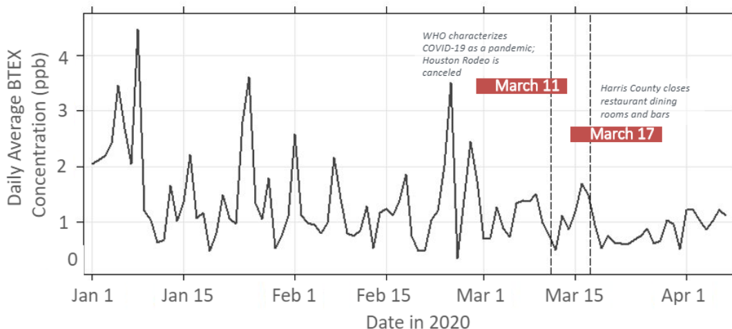
Figure 1. Average daily concentration of BTEX compounds detected in the Houston Ship Channel.
