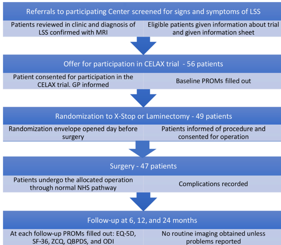
FIG. 3. Trial flowchart. GP = general practitioner. Figure is available in color online only.
