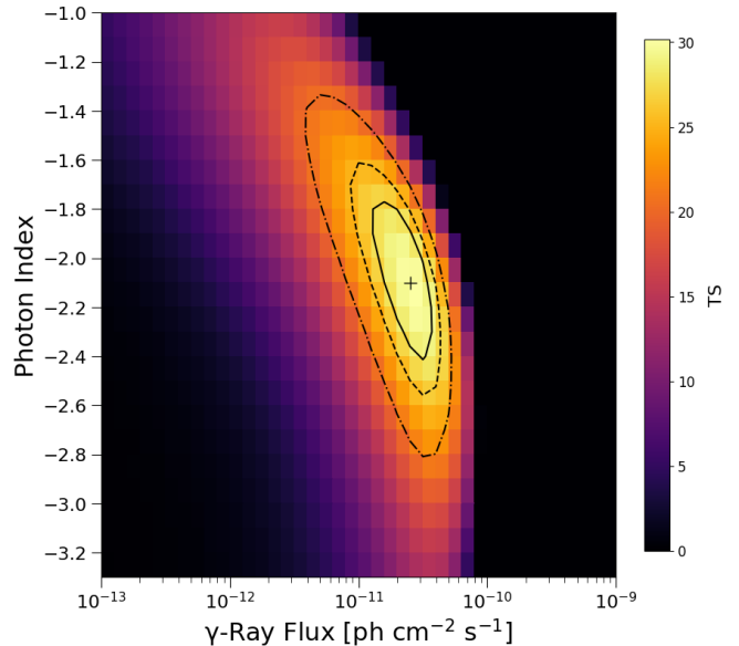
Figure 2. Stacked TS profile for the sample of UFOs. The color scale indicates the TS, and the plus sign indicates the location of the maximum value, with a TS = 30.1 ( 5.1\sigma ). Significance contours (for 2 degrees of freedom) are overlaid on the plot showing the 68%, 90%, and 99% confidence levels, corresponding to \Delta TS = 2.30, 4.61, and 9.21, respectively.
