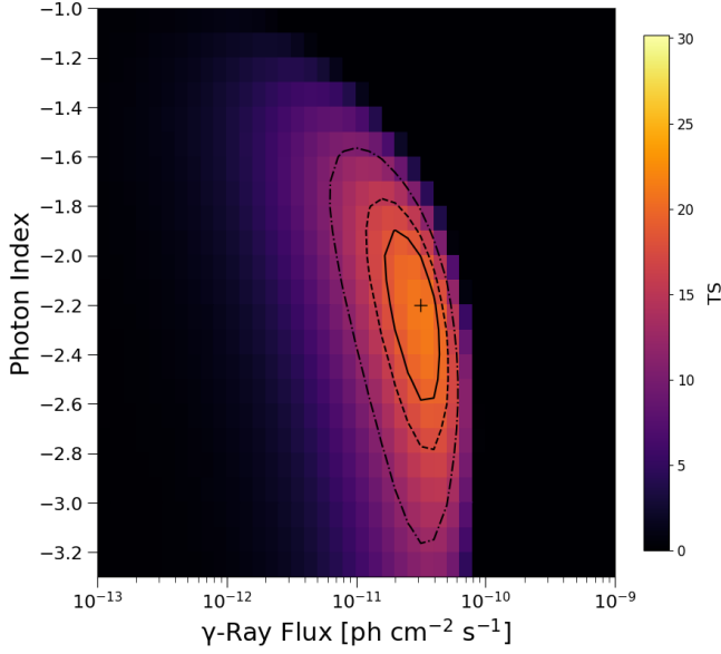
Figure 7. Stacked profile for our simulation run, in which the UFO sources are simulated with an index of -2.1 and a flux of 2.5 \times 10^{-11} \text{ph cm}^{-2} \text{s}^{-1} . The color scale indicates the TS, and the plus sign indicates the location of the maximum value, with a \text{TS} = 21.2 ( 4.2\sigma ). Significance contours (for 2 degrees of freedom) are overlaid on the plot showing the 68%, 90%, and 99% confidence levels, corresponding to \Delta \text{TS} = 2.30 , 4.61, and 9.21, respectively. The maximum TS of the color scale is set to 30.1 (the maximum value from Figure 2).
