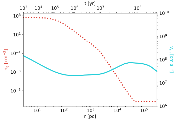
Figure 10. Ambient gas density (red dotted line) and velocity (blue solid line) profiles used in our UFO model. Both profiles come from the models calculated in Liu et al. (2018), for an AGN bolometric luminosity of L_{\text{Bol}} = 2.5 \times 10^{44} \text{ erg s}^{-1} .
