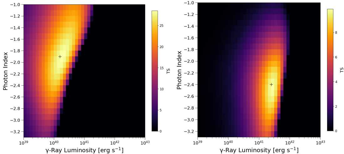
Figure 4. Stacked profiles for bins of bolometric luminosity (the mean kinetic power bins are also the same). The left and the right panels show the stacking for sources with bolometric luminosity (or kinetic power) below and above the average, respectively. The color scale indicates the TS and is set to the maximum value for each bin. The black plus sign gives the best-fit parameters. The first bin consists of 5 sources, with a maximum TS of 28.5 ( 5.0\sigma ); and the second bin consists of 6 sources, with a maximum TS of 9.9 ( 2.7\sigma ).
