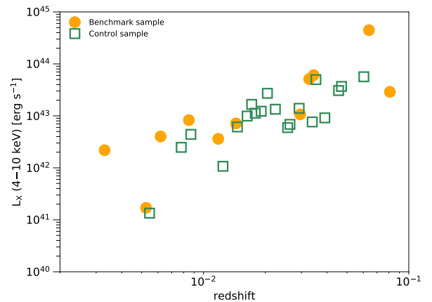
Figure 8. Comparison of redshift and X-ray luminosity ( 4-10 keV) for the control sample and benchmark sample, as indicated in the legend.
