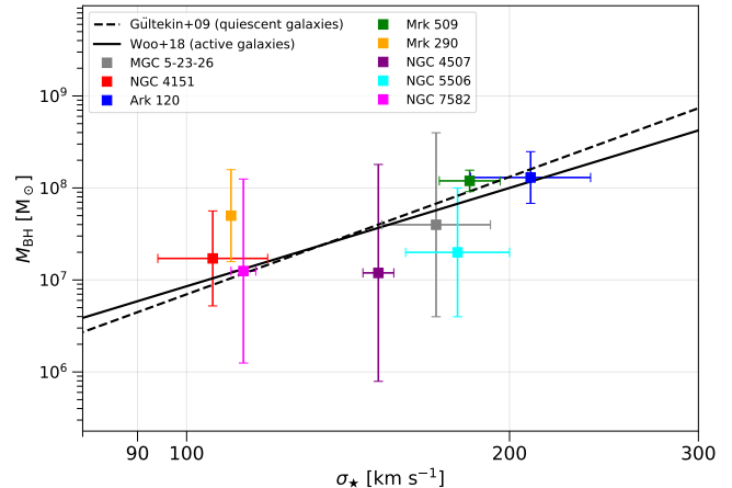
Figure 1. Bulge stellar velocity dispersion versus black-hole mass for our UFO sample, with values taken from the literature. Measurements were found for 8/11 sources. The error bars are statistical plus systematic, where the systematic uncertainty comes from different independent estimates. Information for the velocity dispersion measurements is provided in Table 2. To quantify the systematic uncertainty in the black-hole mass, we use minimum and maximum values from the different references provided in Table 2, as well as the values given in Table 1. The solid and dashed lines show the scaling relations for active and quiescent galaxies, from Woo et al. (2010) and Gültekin et al. (2009), respectively.
