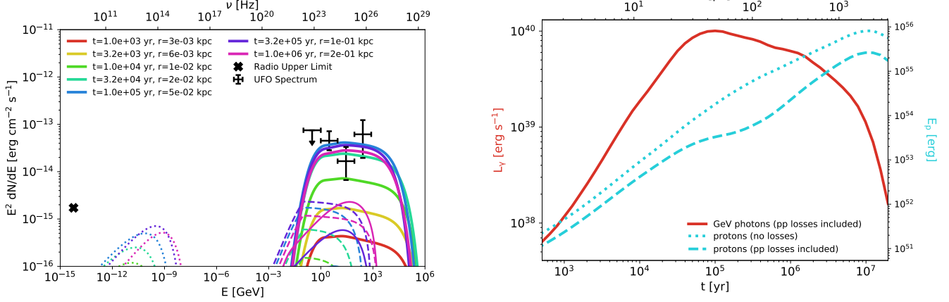
Figure 11. Left: Predicted multiwavelength SED of the UFO’s nonthermal emission as a function of time. Synchrotron emission (dotted curves), bremsstrahlung emission (dashed curves), inverse-Compton emission (thin solid curves) and emission from \pi^0 -decay (thick solid curves) are shown. The inverse-Compton emission remains subdominant despite assuming an artificially enhanced stellar radiation field of energy density 100 eV cm -3 . Also overlaid is the observed \gamma -ray flux as shown in Figure 3 and the average radio upper limit from Table 2. Note that the leptonic emission produced at early times often does not appear as it falls below the plot range. Right: Light curve of a UFO-powered forward shock moving through a representative galaxy. The total energy in CRs is shown before and after proton-proton losses are included (blue dotted and dashed lines, respectively), as is the \gamma -ray luminosity at 1 GeV (red solid line).
