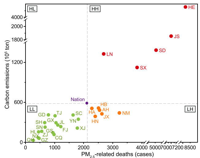
Fig. 7. Four-quadrant distribution of national PM 2.5 -related deaths induced by pollutants emissions in each province and CO 2 emissions of 28 provinces. The coordinate origin represented the national average value (2108, 587) of CO 2 emissions and deaths.
