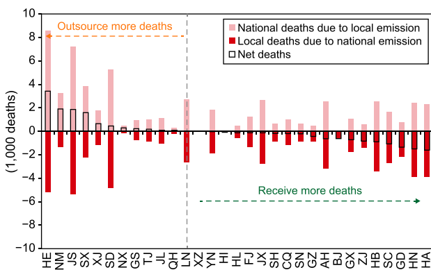
Fig. 6. Provincial PM 2.5 -related deaths incurred by local emissions and transboundary transport of air pollution. Note: local deaths due to all emissions = the deaths in each province due to local emissions and emissions outside the boundary; all deaths due to local emission = the national deaths due to emissions in that province; net deaths = all deaths due to local emission - local deaths due to all emissions.
